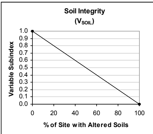
Figure 17. Subindex graphs for low-gradient riverine wetlands (continued)
