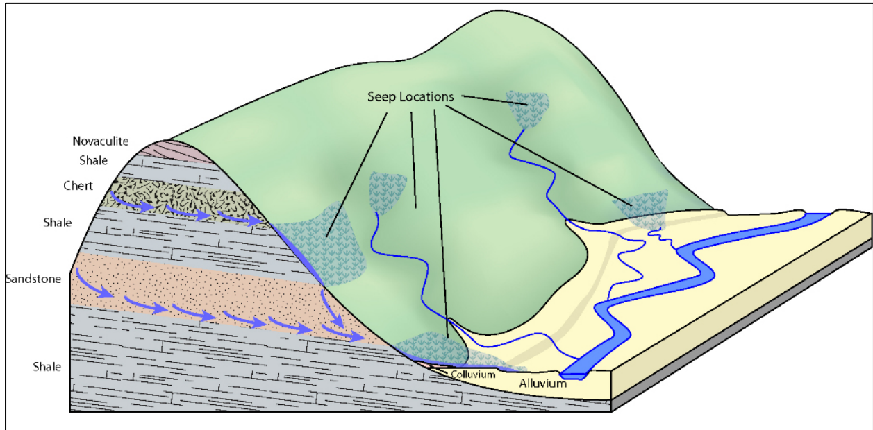
Figure 8. Typical locations of groundwater discharge points (seeps and springs) in the Ouachita Mountains
