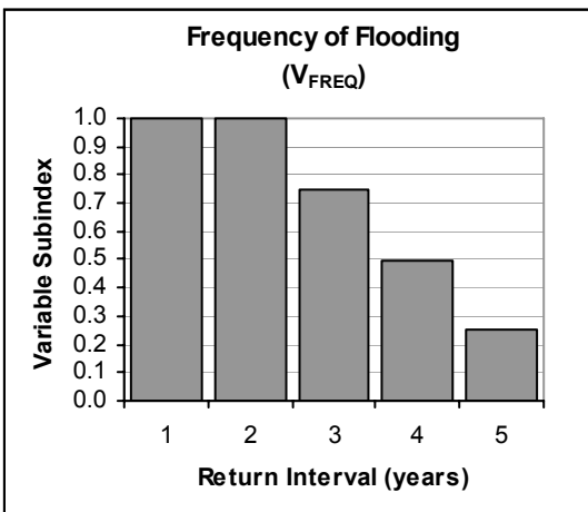
Figure 16. Subindex graphs for mid-gradient riverine wetlands
