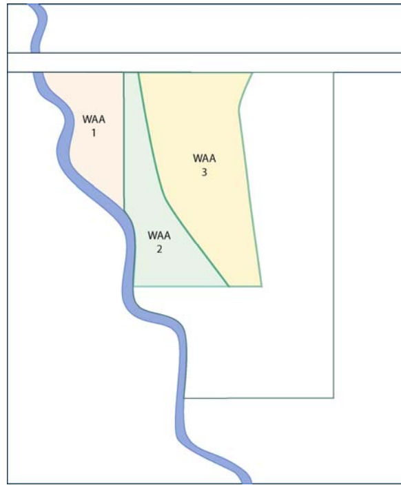
Figure 25. Wetland Assessment Areas
