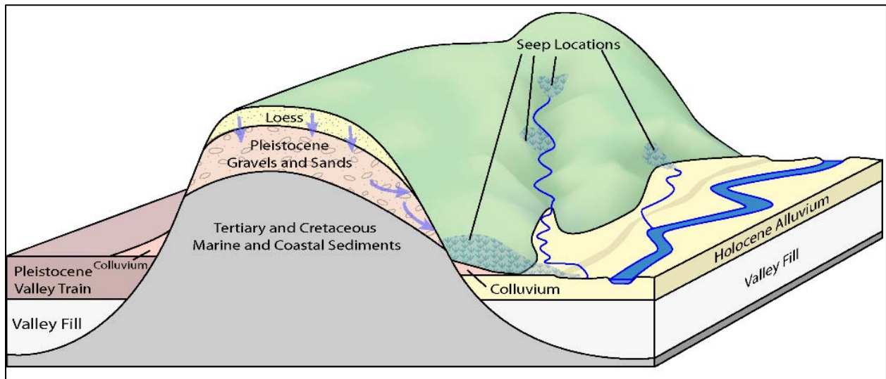
Figure 9. Typical locations of groundwater discharge points (seeps and springs) on Crowley's Ridge
