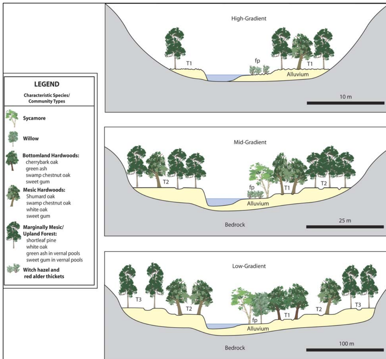
Figure 13. Geomorphic settings and average dimensions of features associated with riverine subclasses in the Ouachita Mountains and Crowley's Ridge Regions. Symbols: fp (floodplain), T1 (terrace 1), T2 (terrace 2), T3 (terrace 3). See Table 5 for additional information
