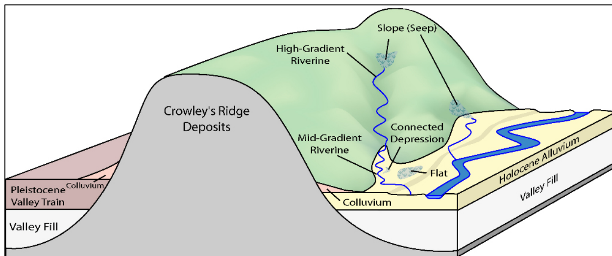
Figure 12. Typical landscape positions of wetland subclasses on Crowley's Ridge.
