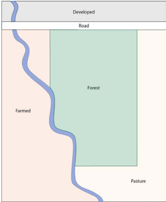
Figure 22. Land cover
