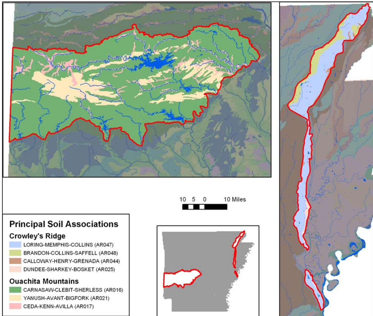
Figure 5. Principal soil associations of the Ouachita Mountains and Crowley's Ridge Regions of Arkansas.
