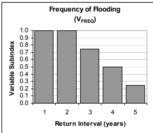
Figure 19. Subindex graphs for connected depression wetlands
