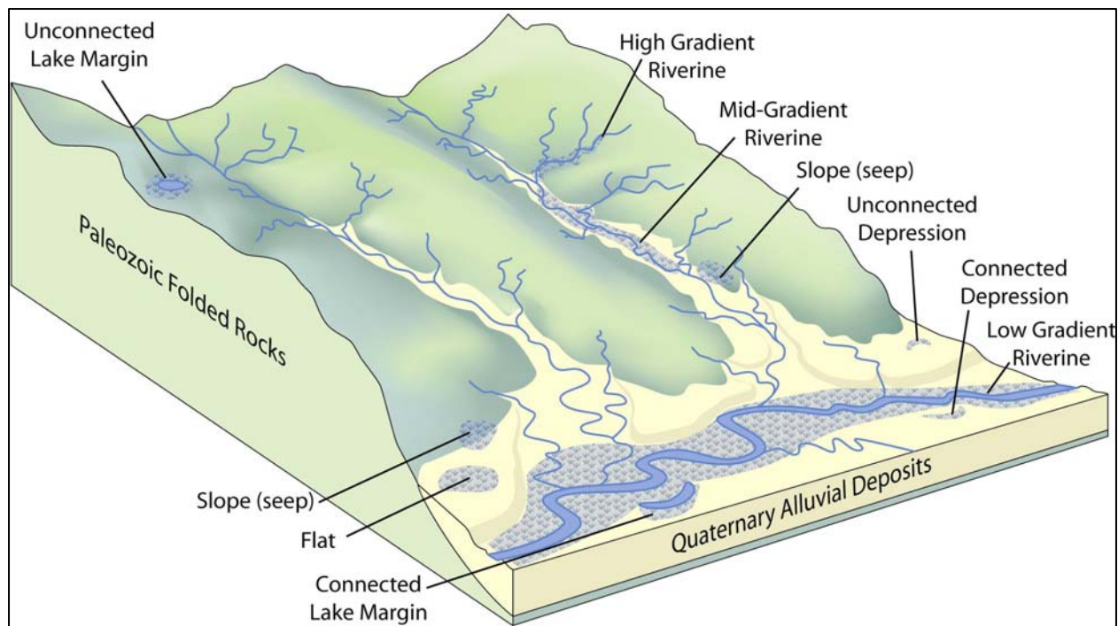
Figure 11. Typical landscape positions of wetland subclasses in the Ouachita Mountains.
