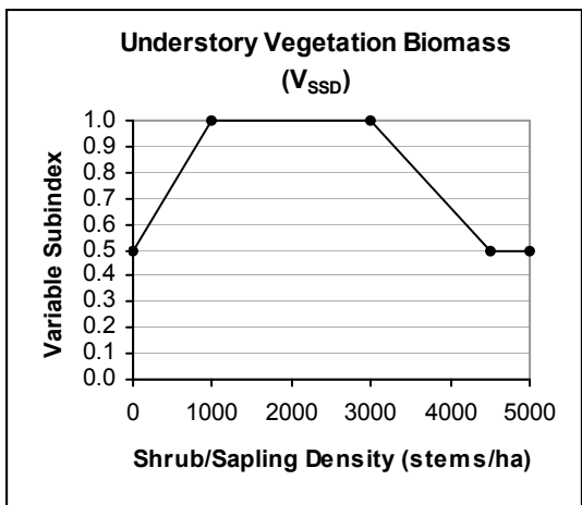
Figure 14. Subindex graphs for flat wetlands (continued)
