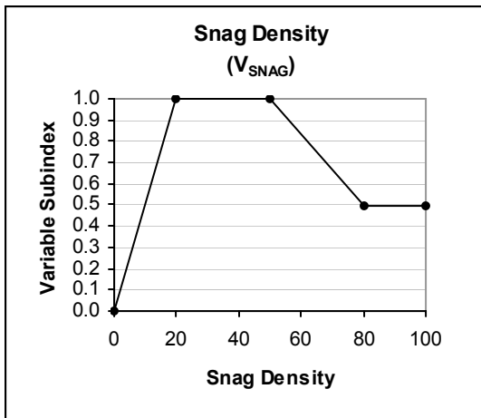
Figure 16. Subindex graphs for mid-gradient riverine wetlands (continued)
