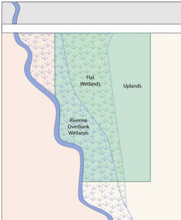
Figure 24. Wetland subclasses
